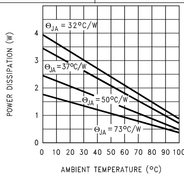
Figure 17. Maximum Power Dissipation (DDPAK/TO-263) (1)
