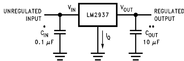
Figure 18. LM2937 Typical Application
